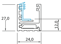
Section aluminum profile
