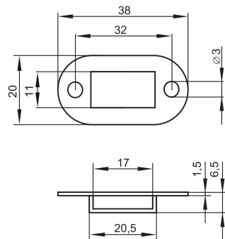
No. # 14.04.091 - 0,37 лв Metal Bar Guide holder for locking bars
