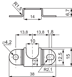
Drawer Stop 913 - A No. # 14.02.030 Left Hand No. # 14.02.020 Right Hand
