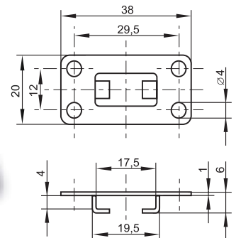
No. # 14.04.091 - 0,37 лв Metal Bar Guide holder for locking bars
